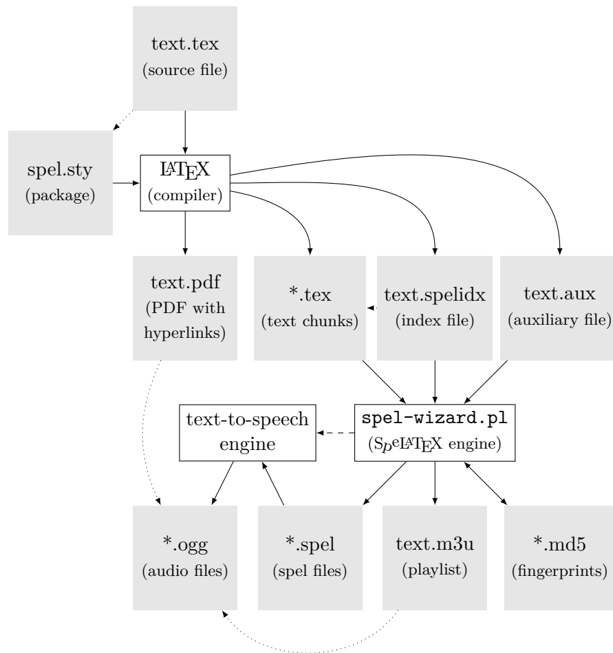
Figure 1: Basic tool setup of the S_{p^e}lA_{T^e}X package; filled boxes indicate files, outlined boxes indicate tools; solid lines indicates use or creation of files, dotted lines indicate references, dashed lines indicate a control relationship.
